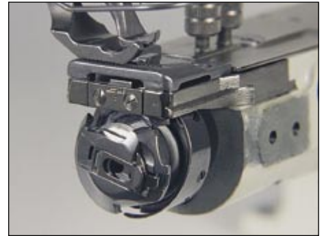
Global® WF1335(B) large bobbin
