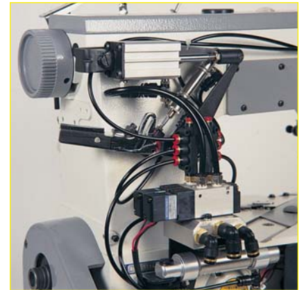
Pneumatic thread trimmer and presser foot lift
