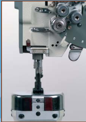
disengageable needle bars (LP 9226 LH-SNB)
